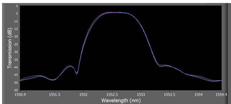
Figure 3 Detailed transmission vs. wavelength data for one channel of the same AWG. The plot shows the maximum, minimum, and average transmission vs. wavelength. The difference between maximum and minimum is an indication of the polarization dependent behavior for this device. The table shows the passband, flatness, and crosstalk information for this channel.
